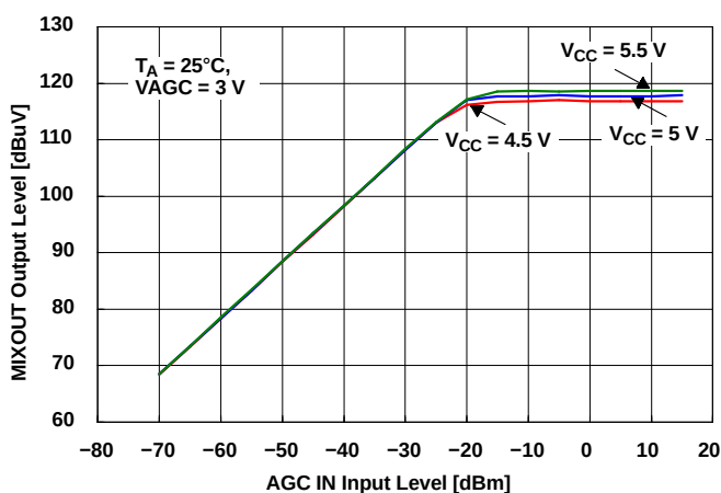
Mixer Output Level vs AGC IN Input Level
